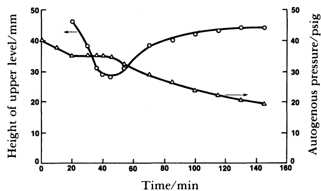
Fig. 1. Profile of autogenous pressure (Δ) and height (○) of product containing layer with time.
